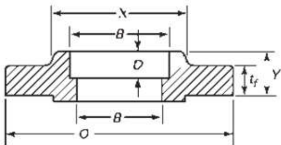
Socket Welding
